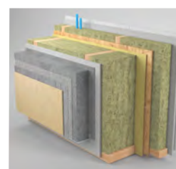
ZID "MEGA" D = 47,80 cm U Wert = 0,082 W/m 2 K
