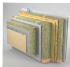
ZID "EURO" D = 36,80 cm U Wert = 0,118 W/m 2 K
