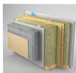
ZID "EURO-MAX" D = 41,00 cm U Wert = 0,094 W/m 2 K
