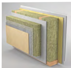
ZID "STANDARD" D = 30,60 cm U Wert = 0,140 W/m 2 K
